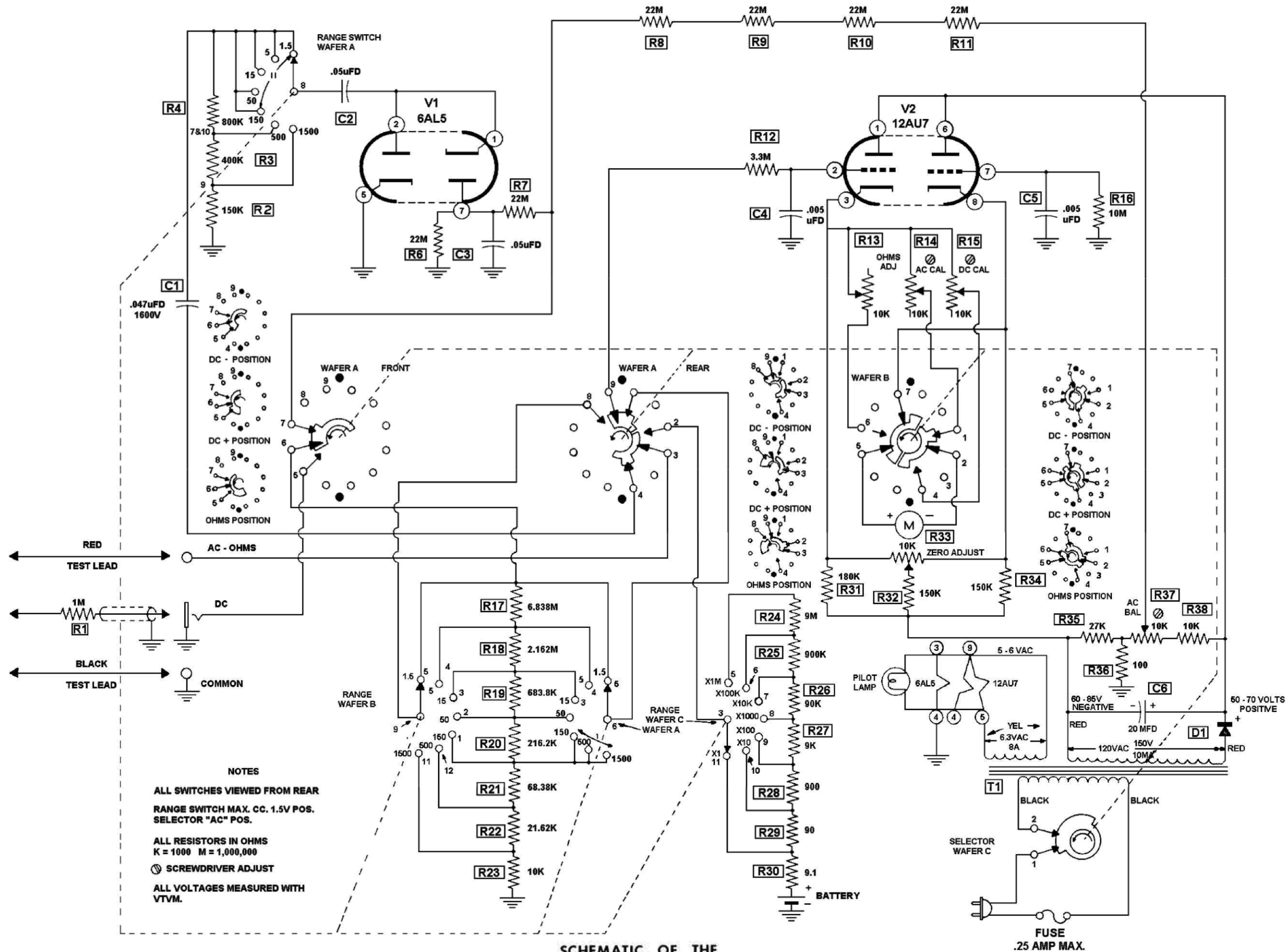
SCHEMATIC OF THE HEATHKIT SERVICE BENCH VTVM MODEL IM-32
