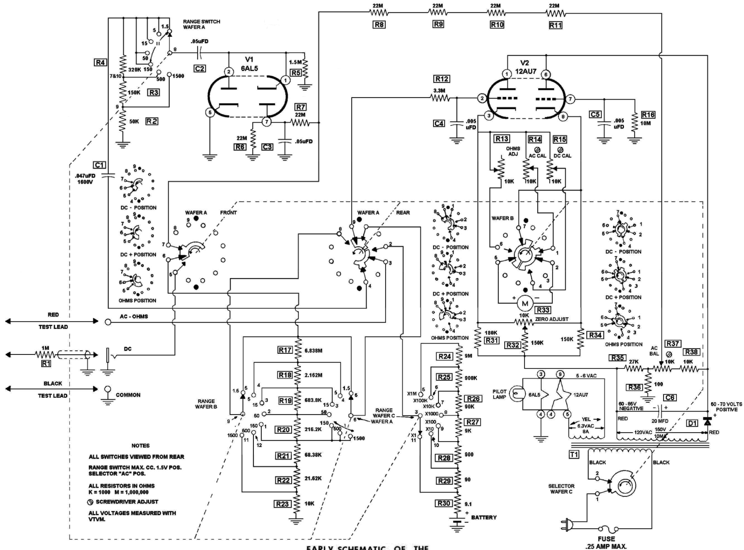
EARLY SCHEMATIC OF THE HEATHKIT SERVICE BENCH VTVM MODEL IM-10
