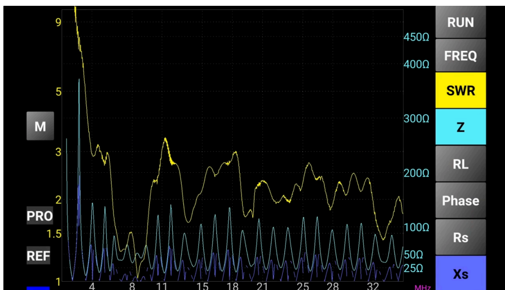
Figure 1 -- KB9RLW Spectrum Plot showing SWR in Yellow
