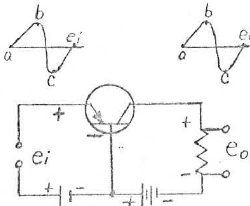
Common Base PNP
