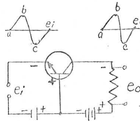
Common Base NPN
