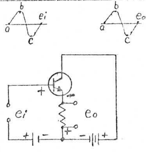
Common Collector NPN
