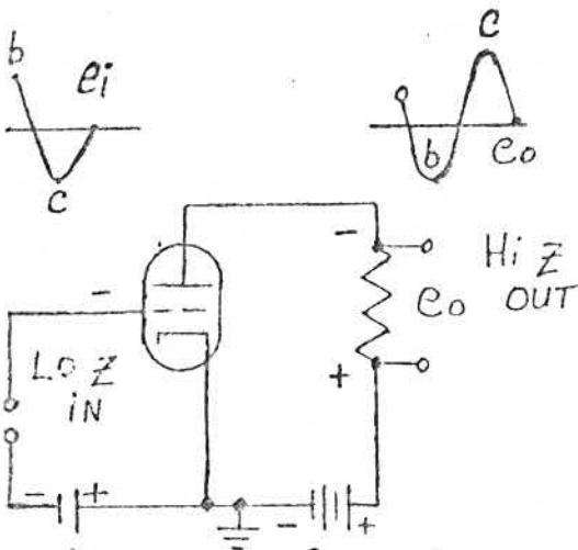
Common Cathode (Grounded Cathode)
