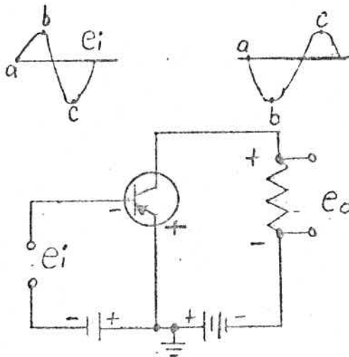
Common Emitter (PNP)
