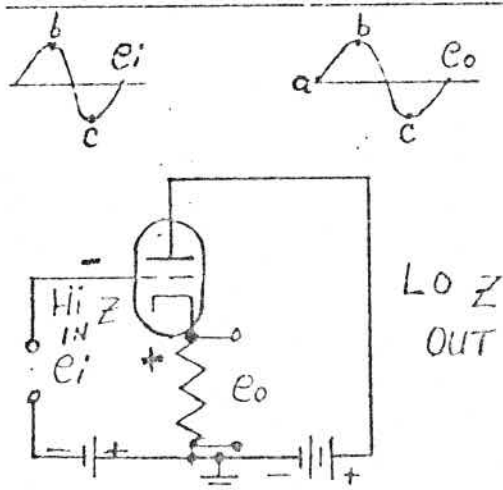
Cathode Follower (Grounded Plate)
