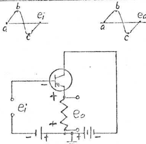
Common Collector PNP
