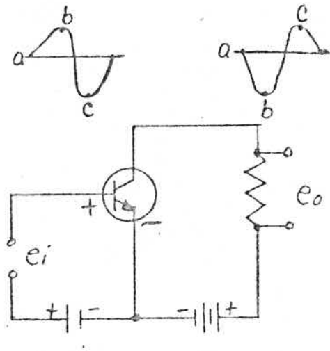
Common Emitter (NPN)
