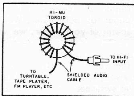
Fig. 20 — The connecting cables between modules of a hi-fi system can be treated with rf chokes by wrapping the shielded audio cable around a high-mu toroid core as shown here. (μ i = 950 to 2000)
